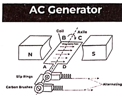
Figure 1: AC Generator
